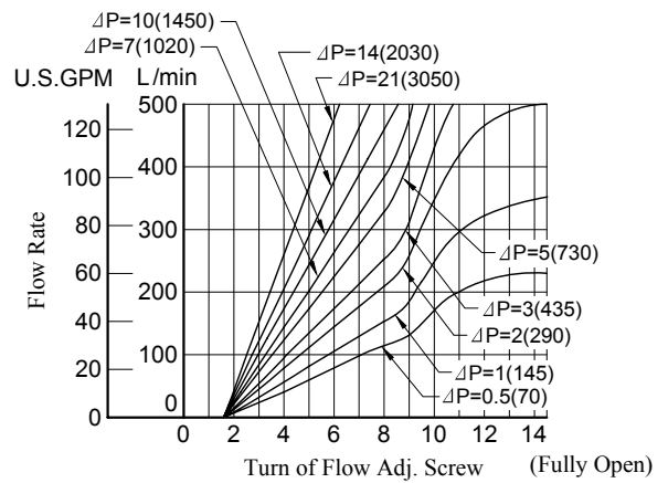
Metred Flow vs. Screw Position
