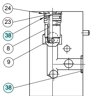
Section Y-Y
